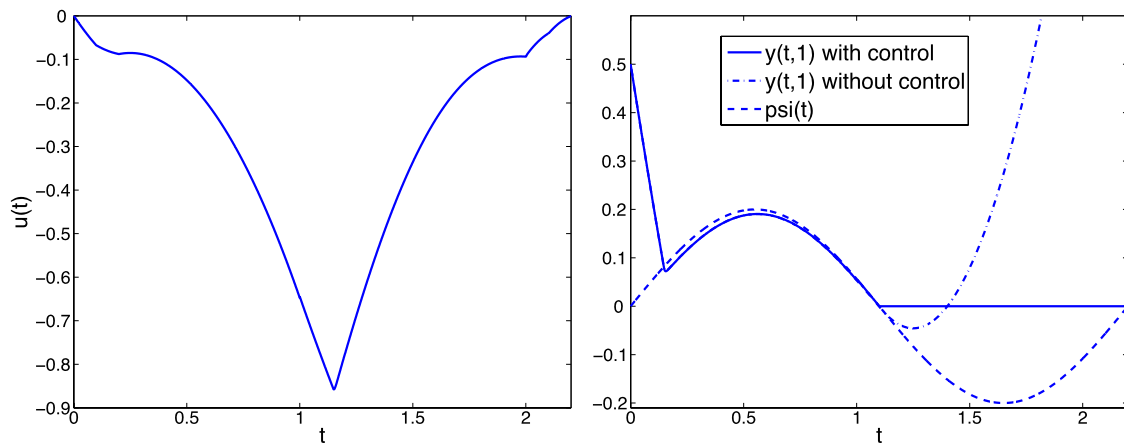
Fig. 3. Penalty method, \epsilon = 1/200 , \psi(t) = \sin(2\pi t/T)/5 . Evolution of the control u_\epsilon (left) and corresponding displacement y_\epsilon(\cdot, 1) (right) vs t \in [0, T] , \|u_\epsilon\|_{L^2(0,T)} \approx 5.533 \times 10^{-1} .
